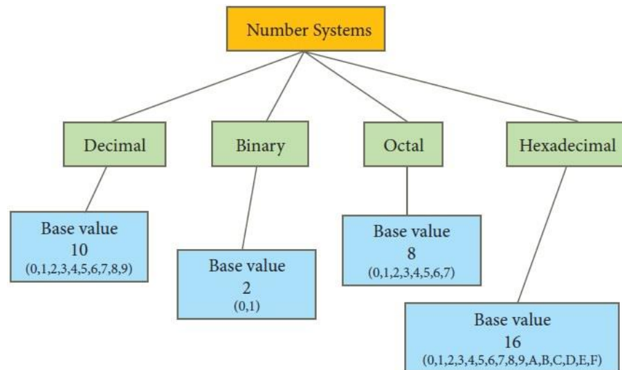
Figure 6: Number System
