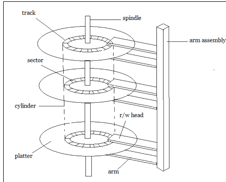
Figure 11: Disk Structure
