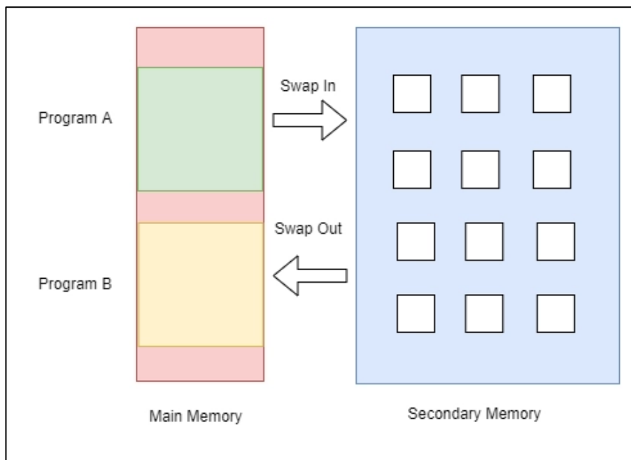
Figure 93: Demand Paging
