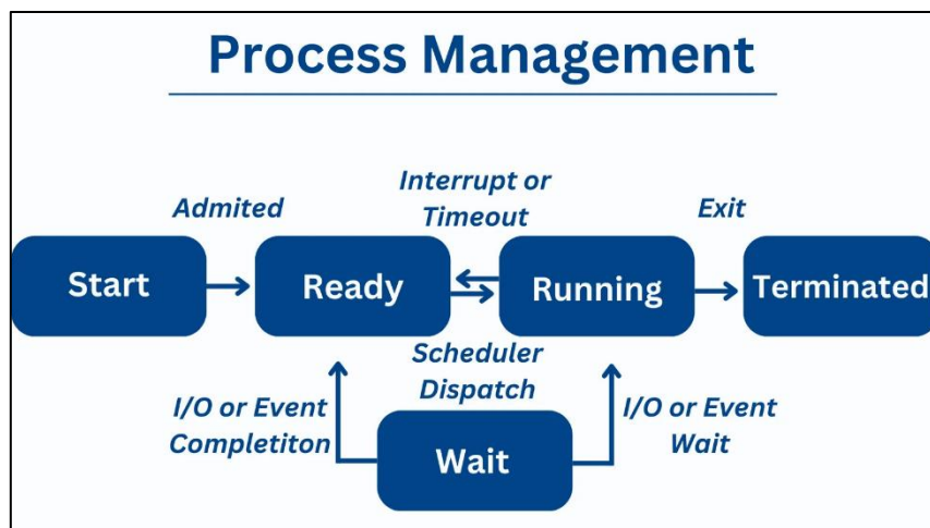
Figure 5: Process Management
