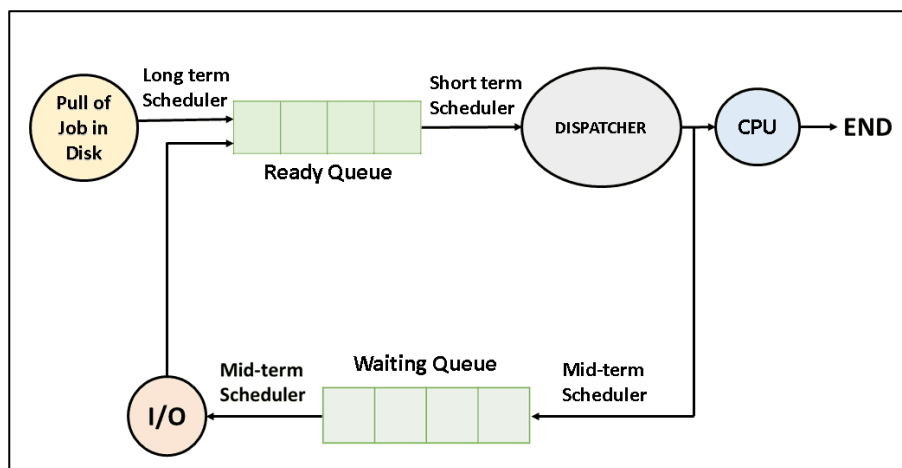
Figure 2.1.4: CPU Scheduling Mechanism
