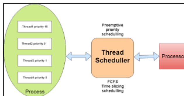
Figure 3: Thread Scheduling
