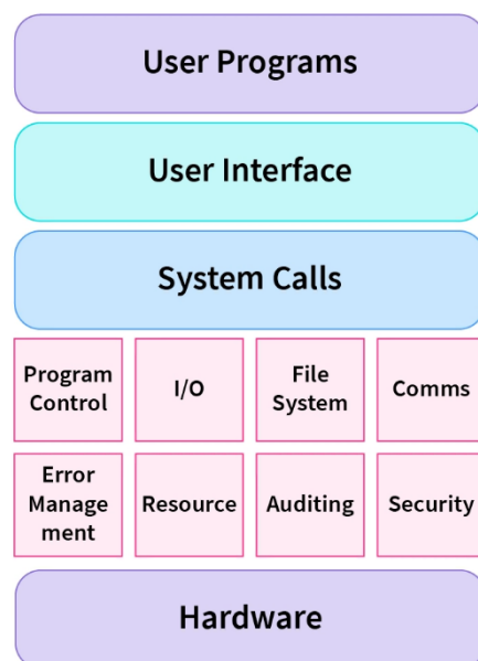
Figure 1.3.9: : System Call [Source - https://www.scaler.com/ ]
