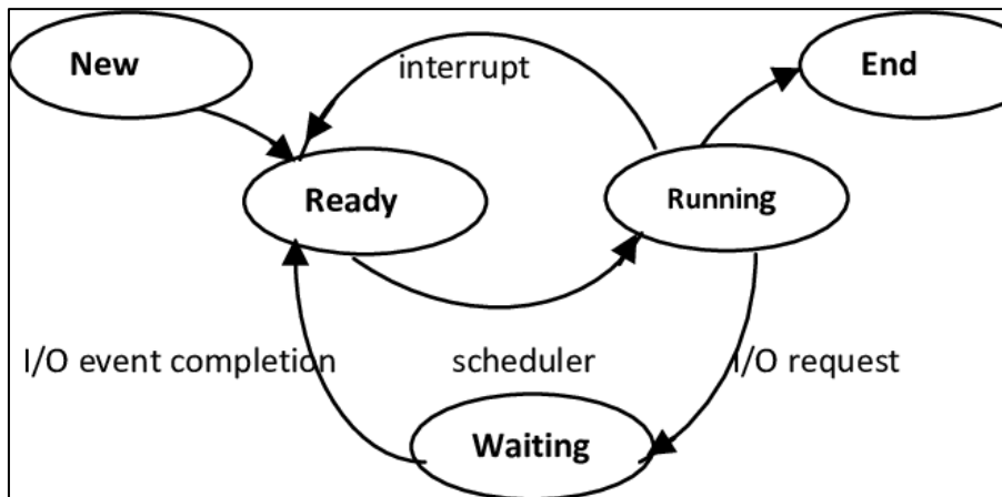
Figure 6: Process State Model [Source - https://www.researchgate.net/ ]
