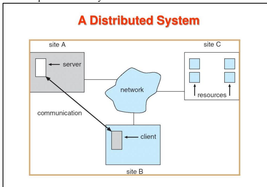
Figure 4.4.6: A Distributed System
