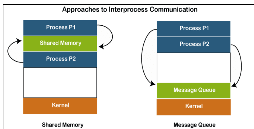
Figure2.1.7: Inter Process Communication
