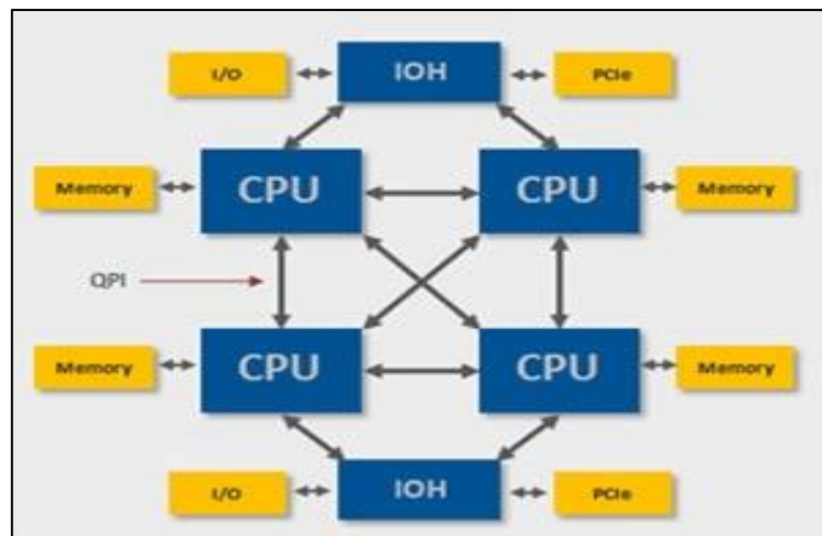
Figure 2.1.3: CPU in Multiprocessing Interface
