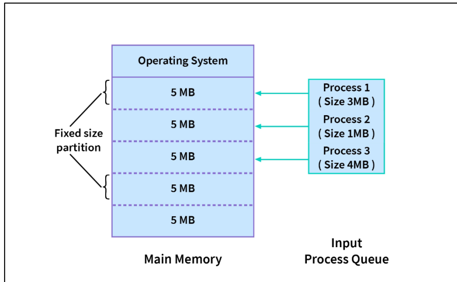
Figure 3.3.17:Contiguous Memory Allocation
