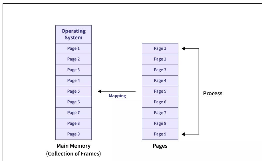
Figure 8: Paging [Source - https://www.scaler.com ]
