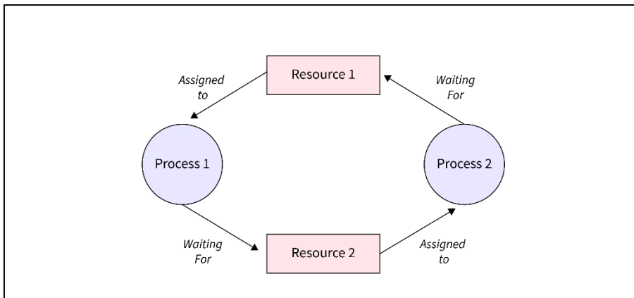
Figure 2.1.12: Deadlock [Source - https://www.scaler.com ]
