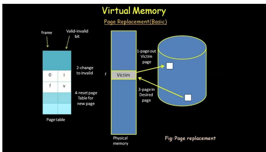
Figure 10: Page Replacement Concept
