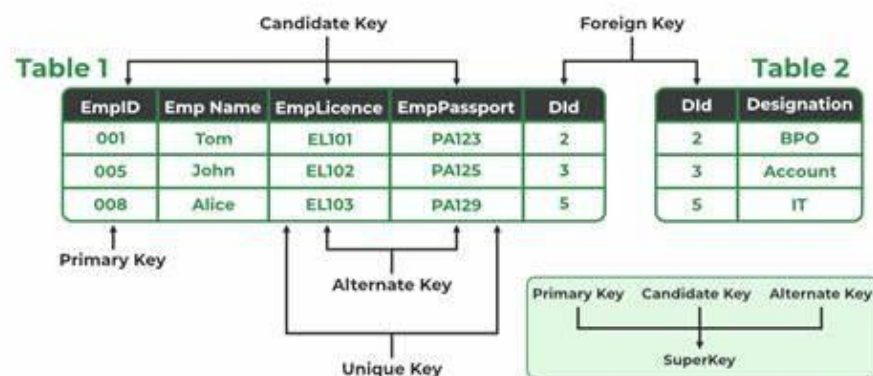
Figure 10: Keys in Database System
