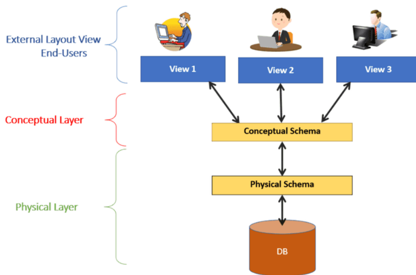
Figure 7: Database Schema [Source: https://estuary.dev/ ]
