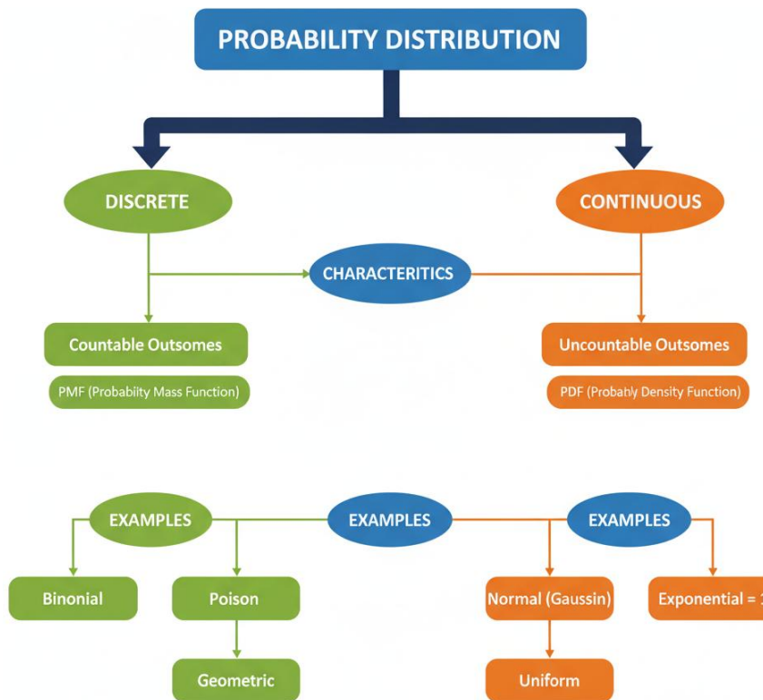
Figure 3.2 Probability Distribution
