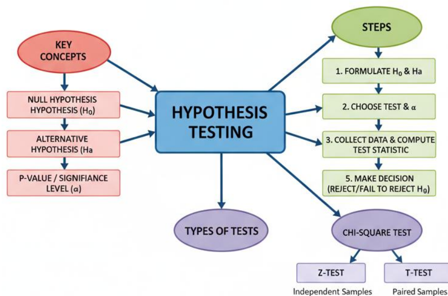
Figure 3.3 Hypothesis Testing
