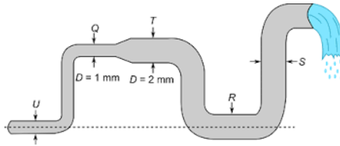
Figure 1.1 [Diagram showing pipes at different heights and diameters]
