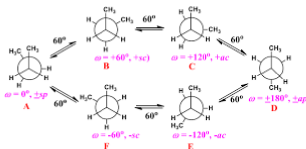
Fig. 2.2 Conformational Structures of n-Butane
