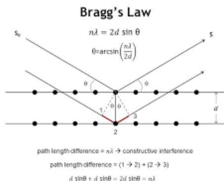
Fig. 3.2 Bragg's law
