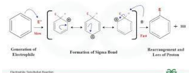
Fig 2.1 Electrophilic Substitution
