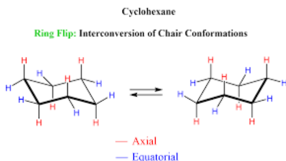
Fig. 2.3 Conformational Structures of Cyclohexane
