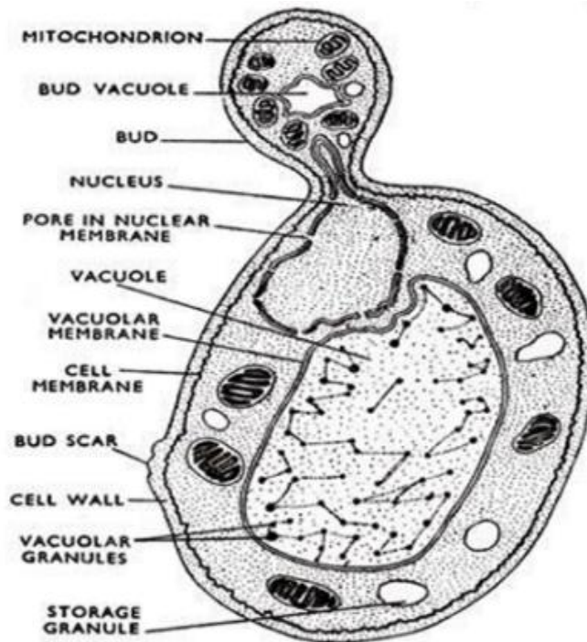
Fig. 2.4 Cell Structure
