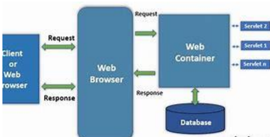
Figure 3.1.1: Servlet Architecture [ Source: https://th.bing.com/ ]
