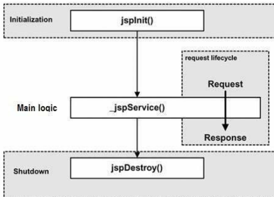
Figure 4.1.1: JSP Life Cycle
