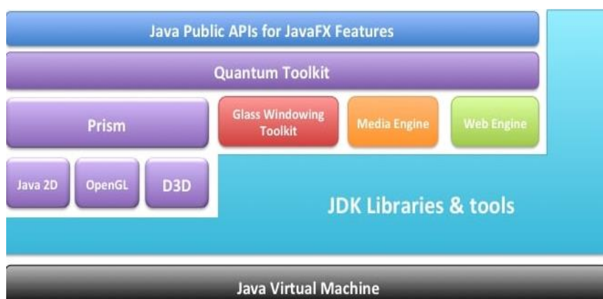
Figure 2.1.5: JavaFX Architecture
