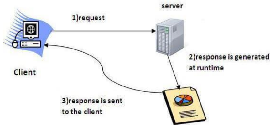
Figure 3.2.1: Servlet
