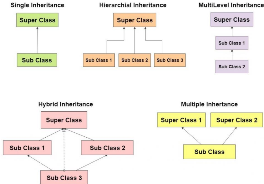
Figure1.1.4: Types of Inheritance [Source: https://www.acte.in/ ]
