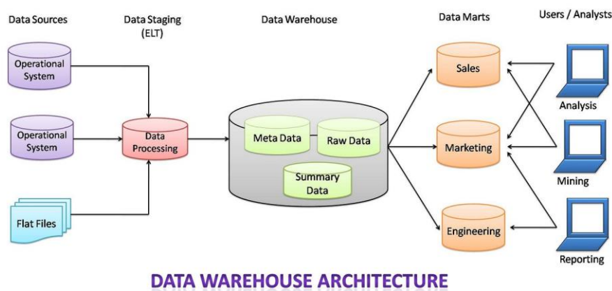
Figure 1.2.2: Data warehouse [Source: https://medium.com/ ]
