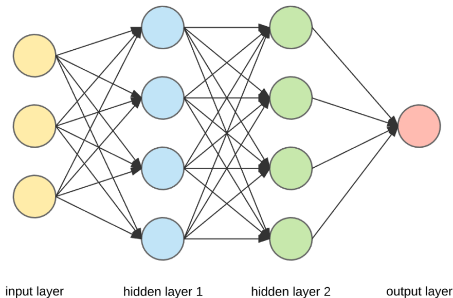
Figure 1.1.2: Neural Network
