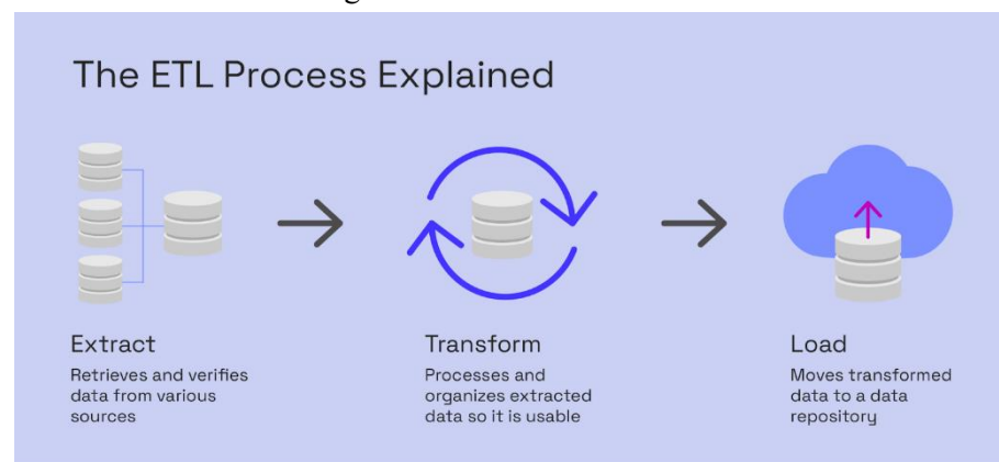
Figure 3.1.1: ETL Process
