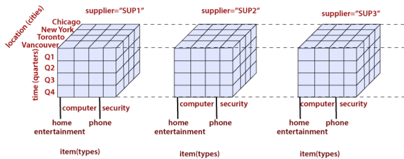
Figure 3.2.2: Data Cube Example
