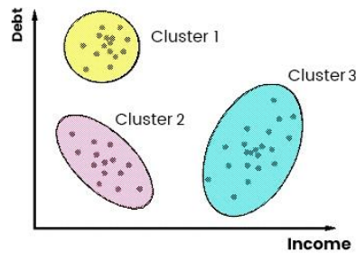
Figure 5.31: Cluster Analysis
