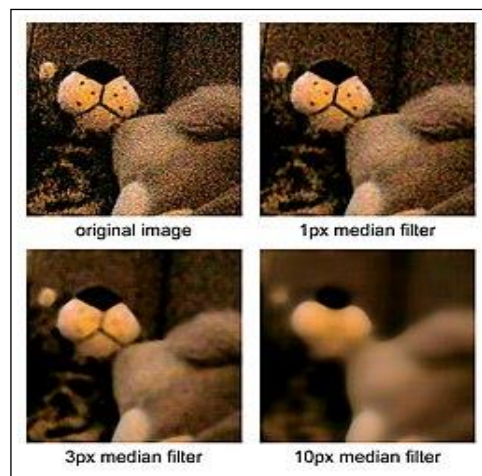
Figure 3.2.3: Median Filtering
