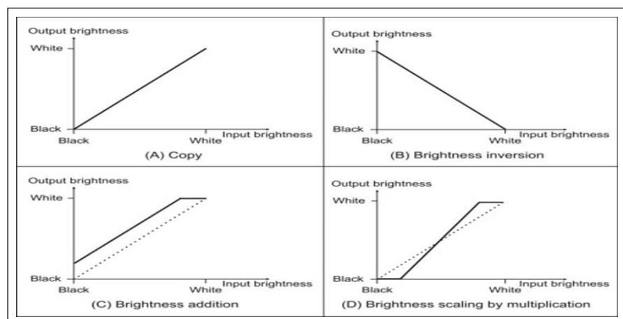
Figure 2.1.1: Overview of Point Processing Operations
