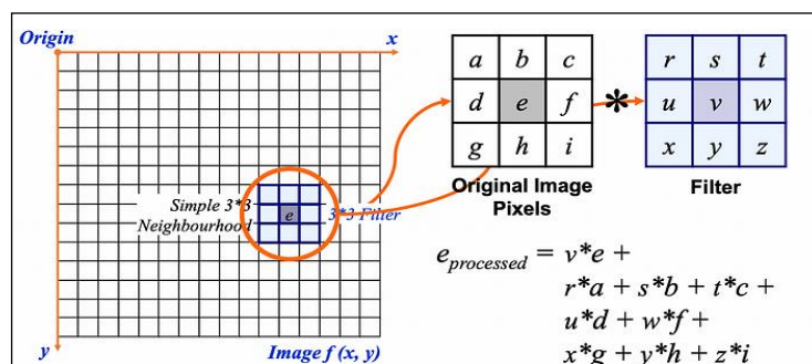
Figure 2.2.1: Overview of Spatial Filter
