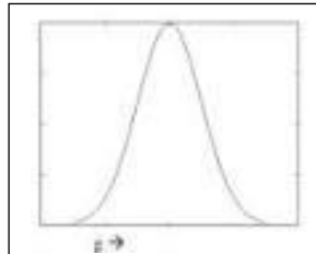
Figure 3.2.1: Gaussian noise
