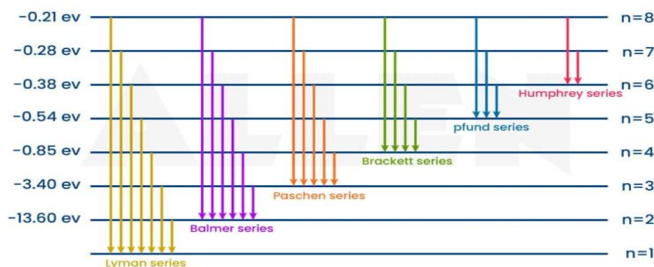
Figure 2.1 The hydrogen atom's spectrum
