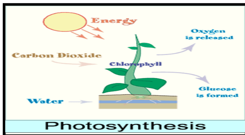
Fig.1.2.1. Phytosynthesis
