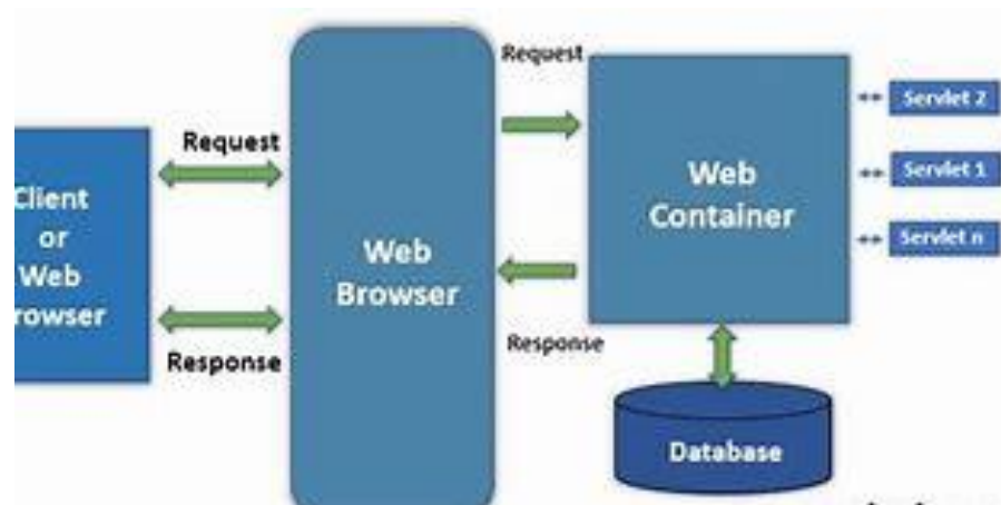
Figure 5.1: Servlet Architecture
