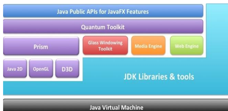
Figure 2.1: JavaFX Architecture
