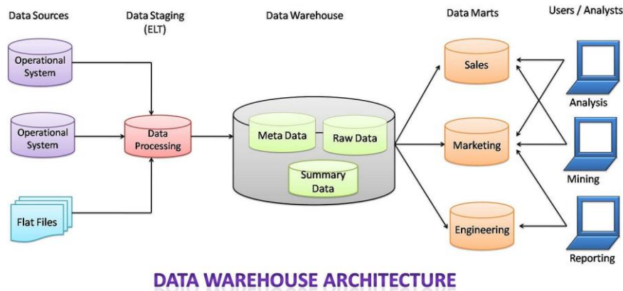
Figure 4: Data warehouse [Source: https://medium.com/ ]
