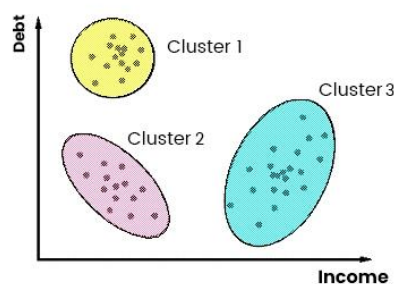
Figure 11: Cluster Analysis
