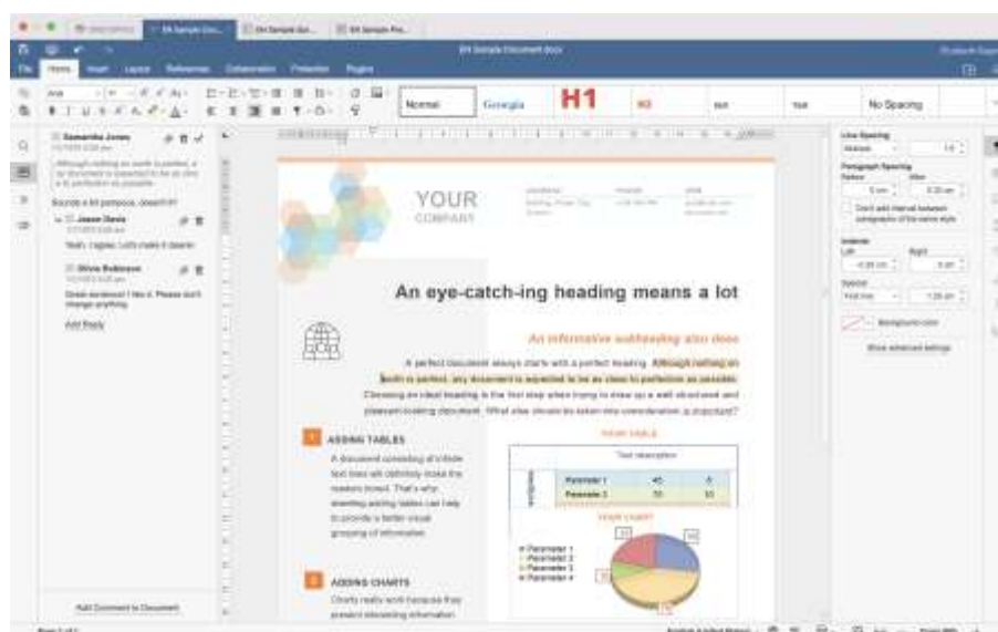
Figure 1: Word Documentation
