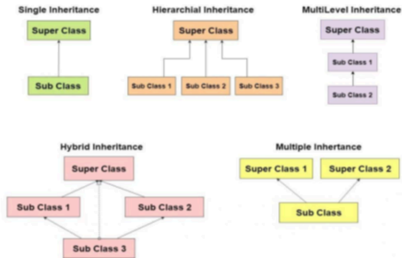
Figure 4: Types of Inheritance
