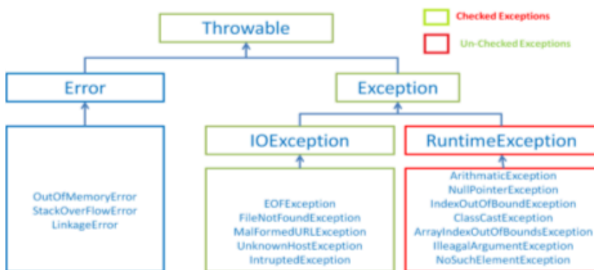
Figure 1.4: Exception Hierarchy [Source: https://th.bing.com/ ]
