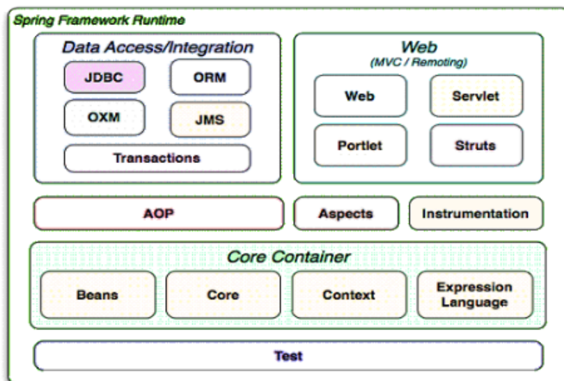
Figure 5.1: Spring Framework [Source: https://www.careerride.com/ ]
