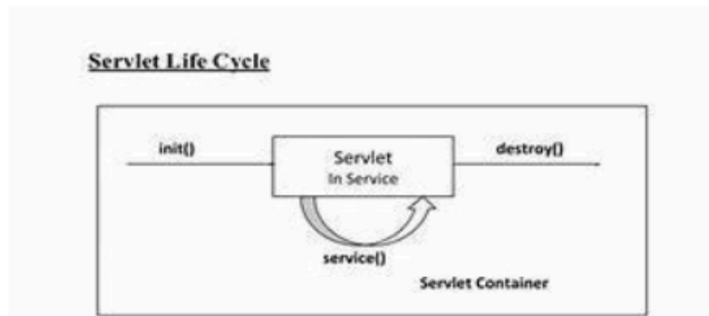
Figure 3.2: Servlet Life Cycle [Source: https://th.bing.com/ ]
