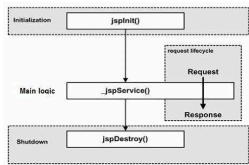
Figure 4.1: JSP Life Cycle [Source: https://www.researchgate.net/ ]
