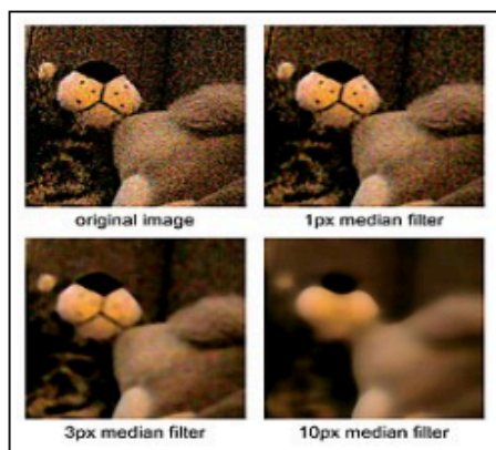
Figure 18: Median Filtering
