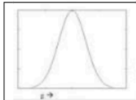
Figure 16: Gaussian noise
